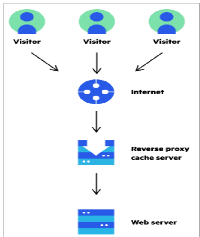
Fig. 6 Server caching
